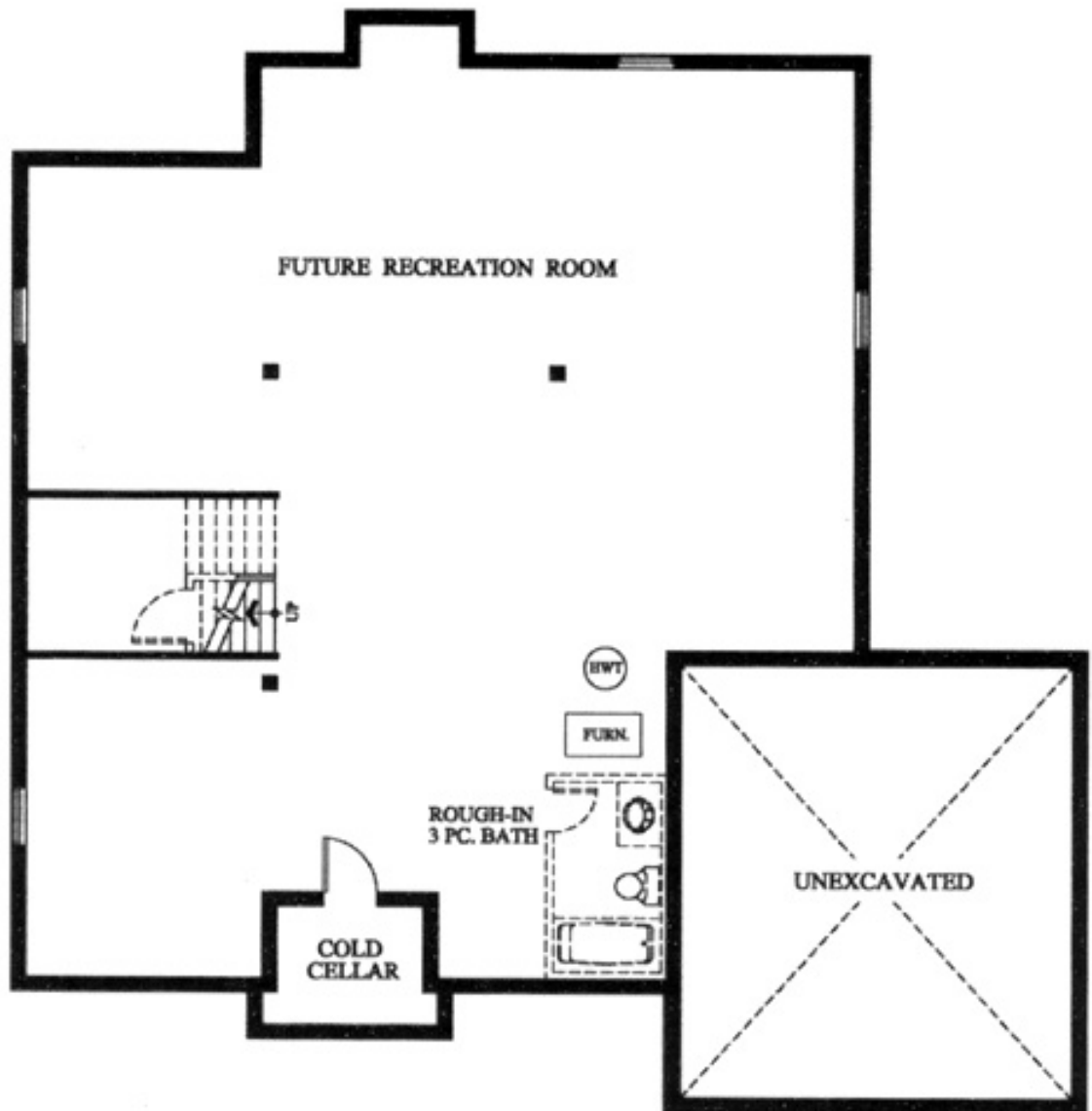
Basement Plan
