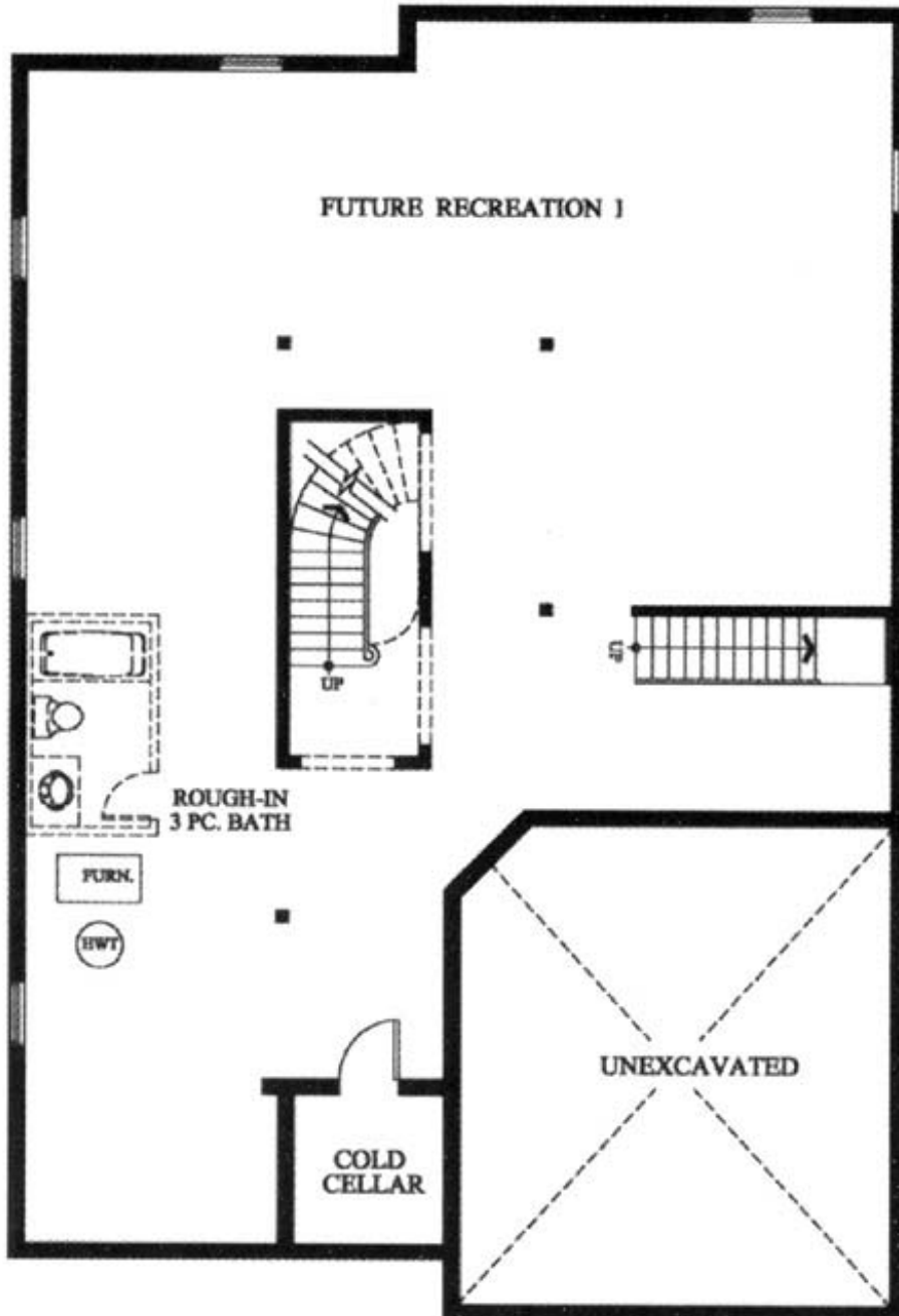
Basement Plan
