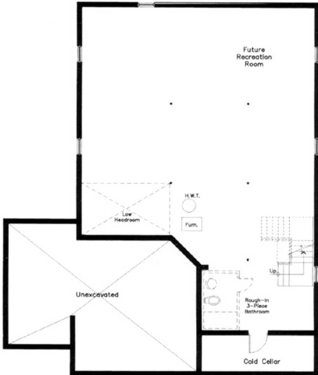
Basement Plan
